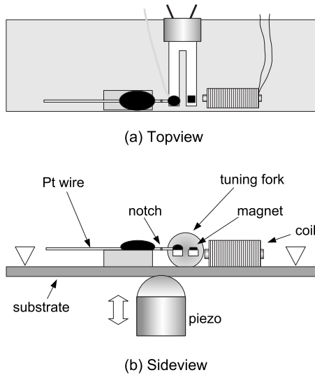
FIG. 1. Schematics of (a) a top view and (b) a side view of our MCBJ system with a tuning fork as a force sensor. See text for further details.
